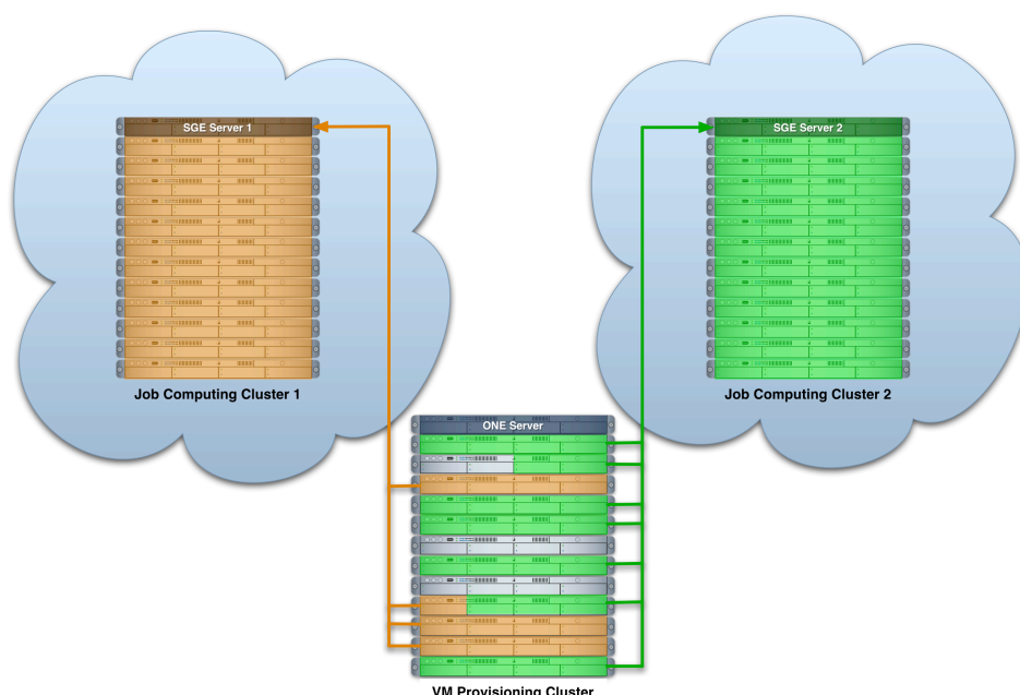
Dynamic cluster partitioning to execute different service workloads
